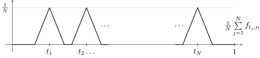
FIGURE 2. Convex combination of f_{t_j, n} with arbitrarily small norm.
