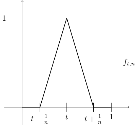
FIGURE 1. The graph of the function f_{t,n} .
