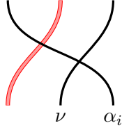
FIGURE 3. An example of an element of the violating ideal.
