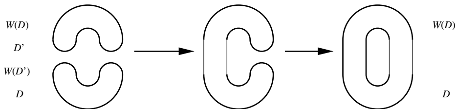
FIGURE 3. Composition of maps: R \otimes R \xrightarrow{m} R \xrightarrow{\Delta} R \otimes R .
