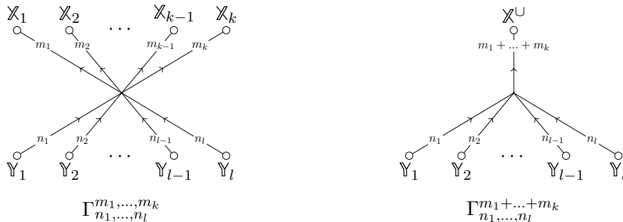
Figure 12: Comparison of two basic MOY-graphs
