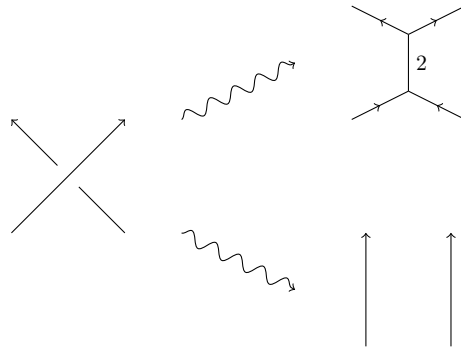
Figure 6: Resolving a crossing
