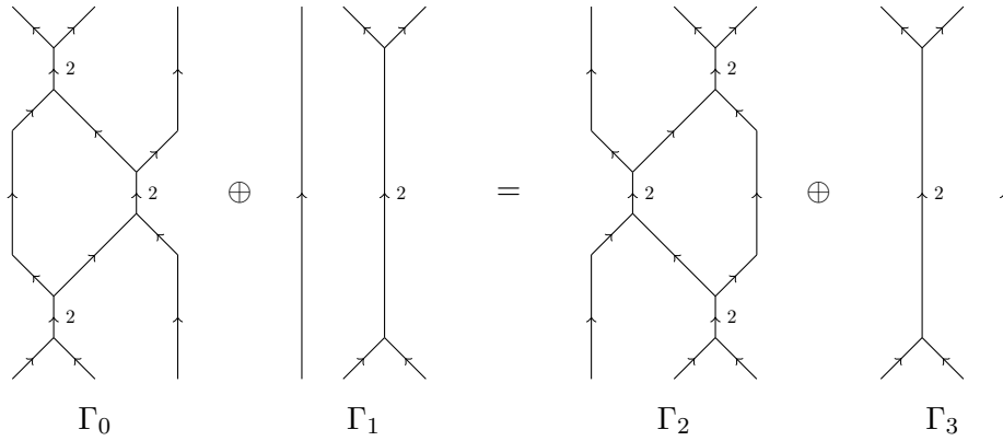
Figure 18: Basic MOY-relation
