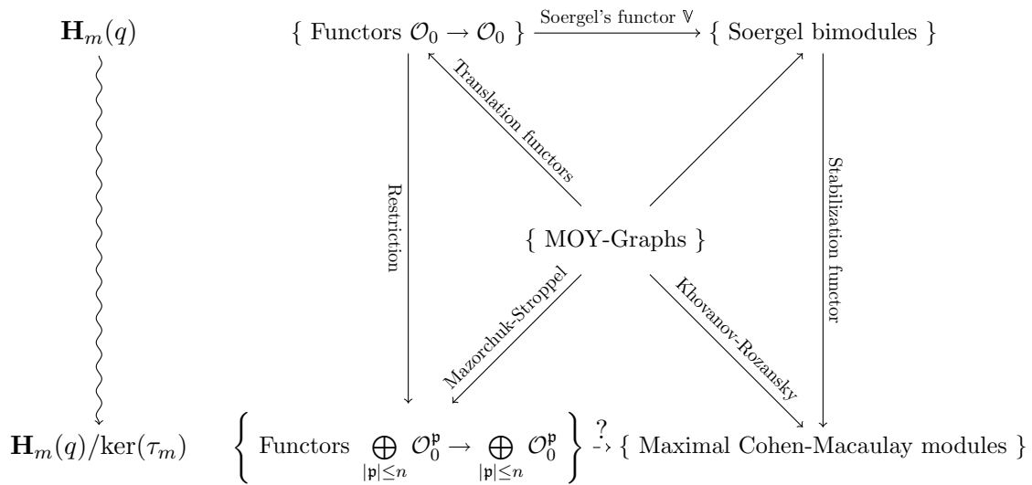
Figure 10: Overview over the results of this work.
