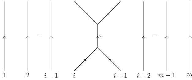
Figure 17: Basic MOY-braid \sigma_i
