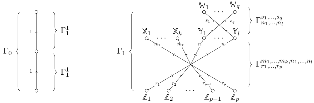
Figure 13: Gluing two basic MOY graphs
