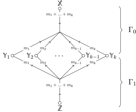
Figure 15: \Gamma
