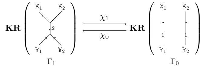
Figure 19: \chi -morphisms
