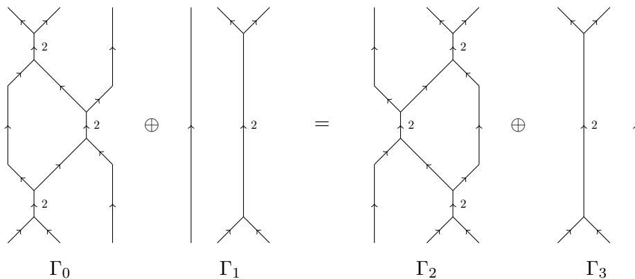
Figure 9: Basic MOY-relation
