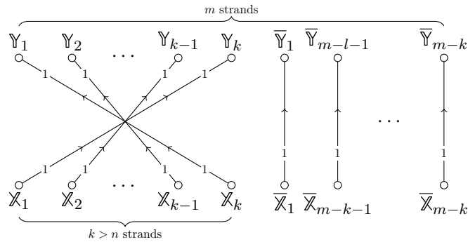
Figure 20: MOY-graph with trivial matrix factorization
