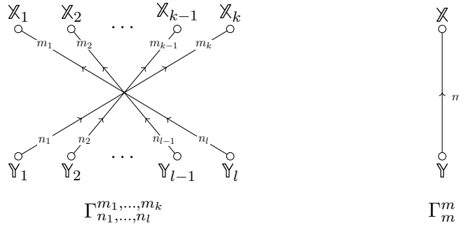
Figure 11: Building blocks
