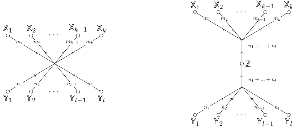
Figure 14: Decomposition of \Gamma_{n_1, \dots, n_l}^{m_1, \dots, m_k} into \Gamma_{n_1, \dots, n_l}^{n_1 + \dots + n_l} and \Gamma_{n_1 + \dots + n_l}^{m_1, \dots, m_k} .
