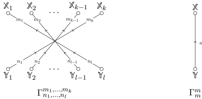
Figure 7: Building blocks
