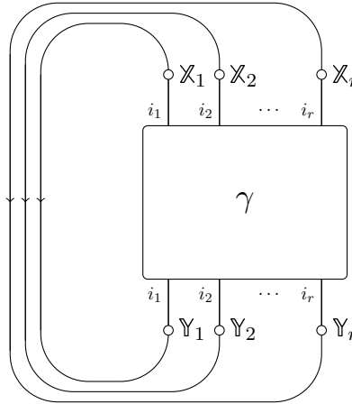
Figure 21: Closure of a braid
