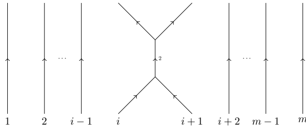
Figure 8: Basic MOY-braid \sigma_i
