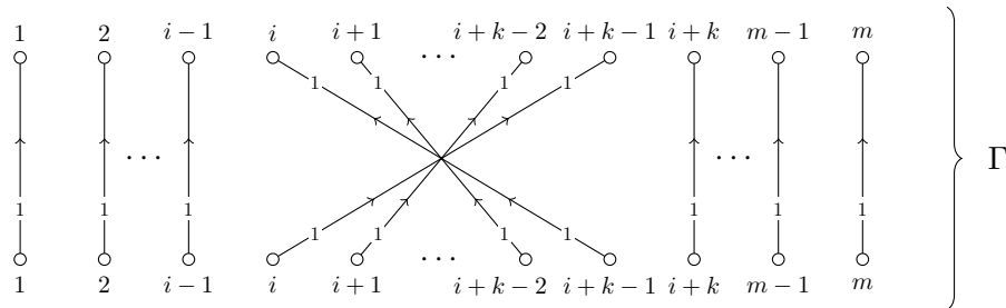
Figure 16: Another basic MOY-graph
