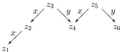
FIGURE 1. The string module M(xxyxy)
