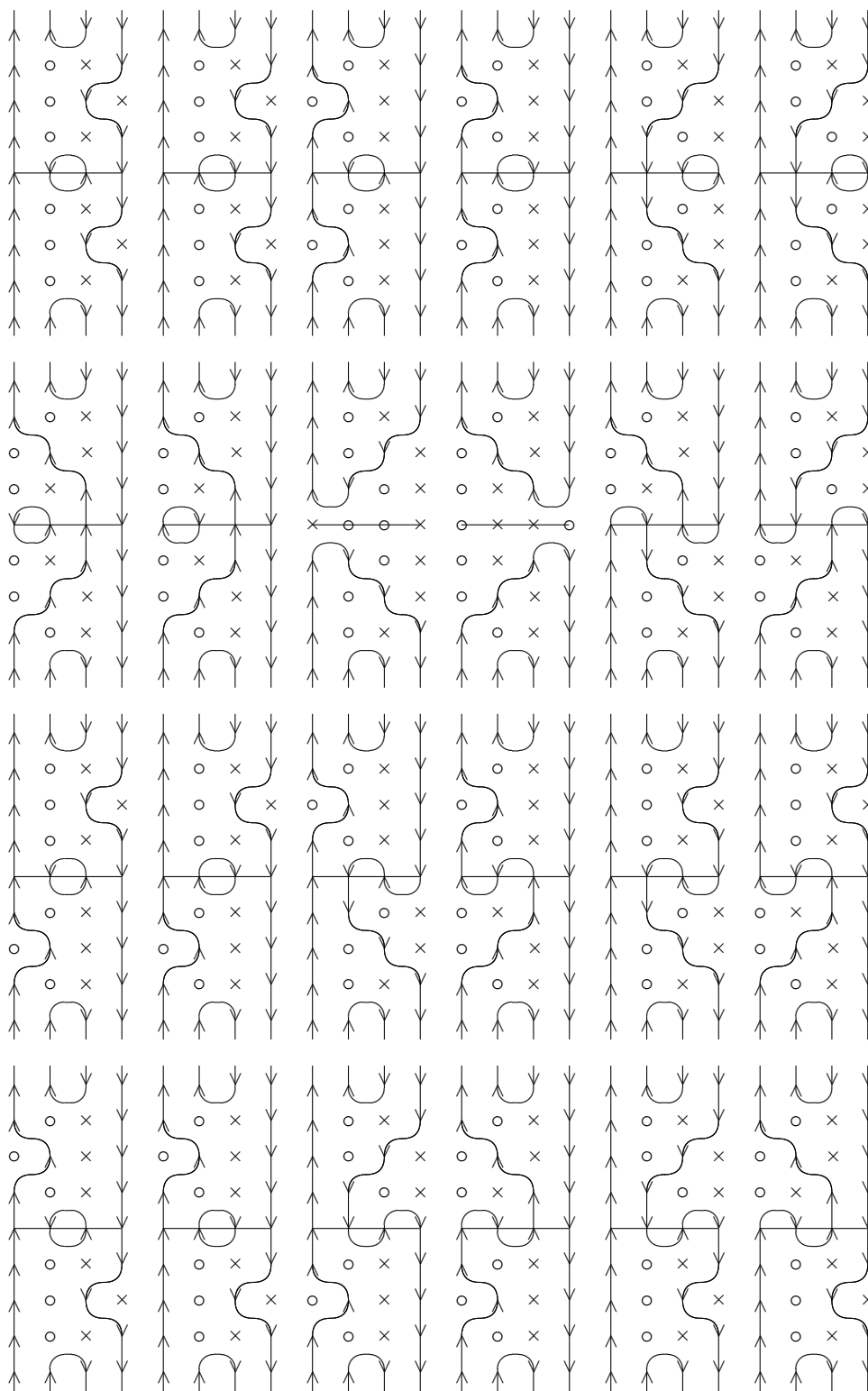
FIGURE 1. The diagram basis for B_{E^2 F^2}(0)
